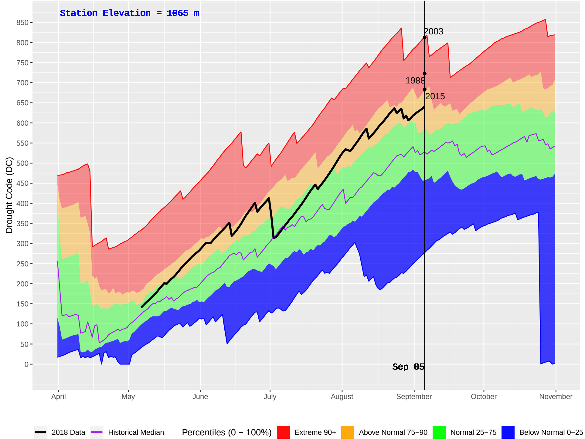
PLACE LAKE (212) : Historical (1981–2016) and Current (2018) Daily Drought Code (DC)
