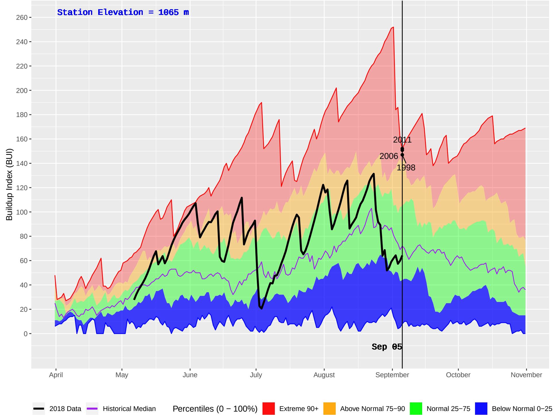
PLACE LAKE (212) : Historical (1981–2016) and Current (2018) Daily Buildup Index (BUI)
