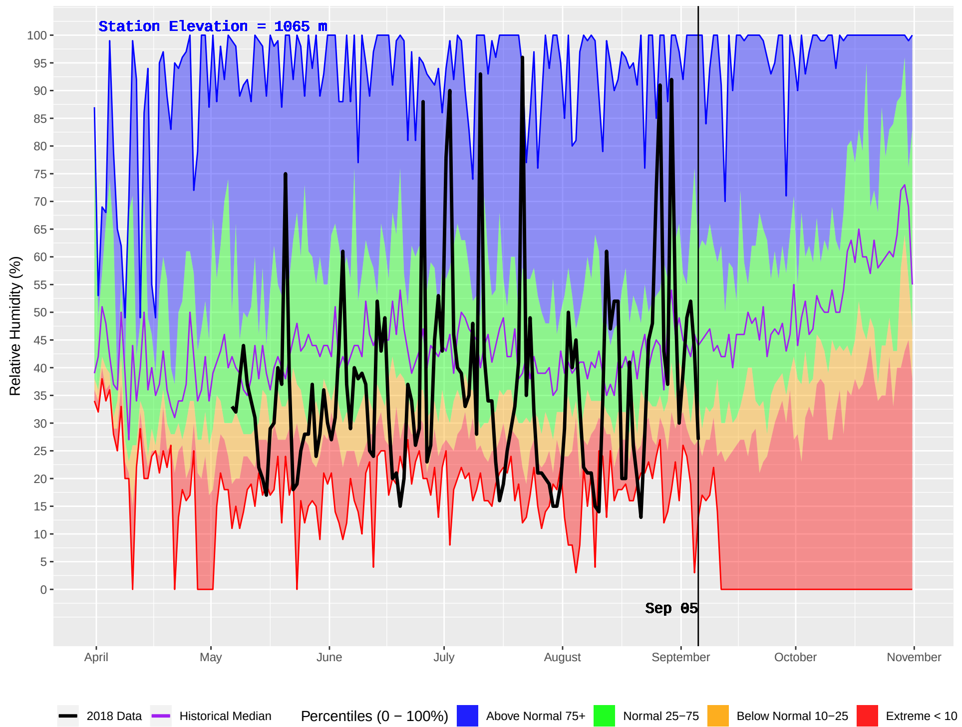
PLACE LAKE (212) : Historical (1981–2016) and Current (2018) Daily Relative Humidity
