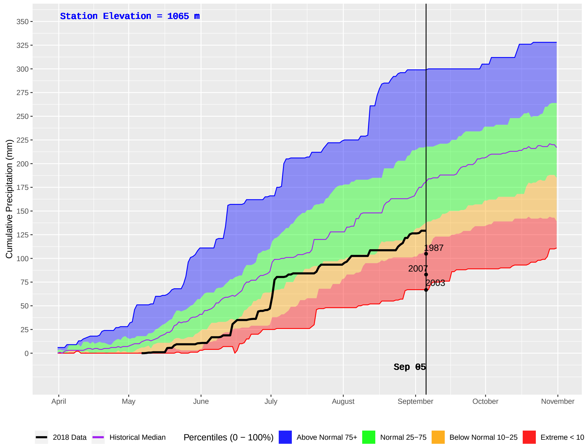
PLACE LAKE (212) : Historical (1981–2016) and Current (2018) Daily Cumulative Precipitation
