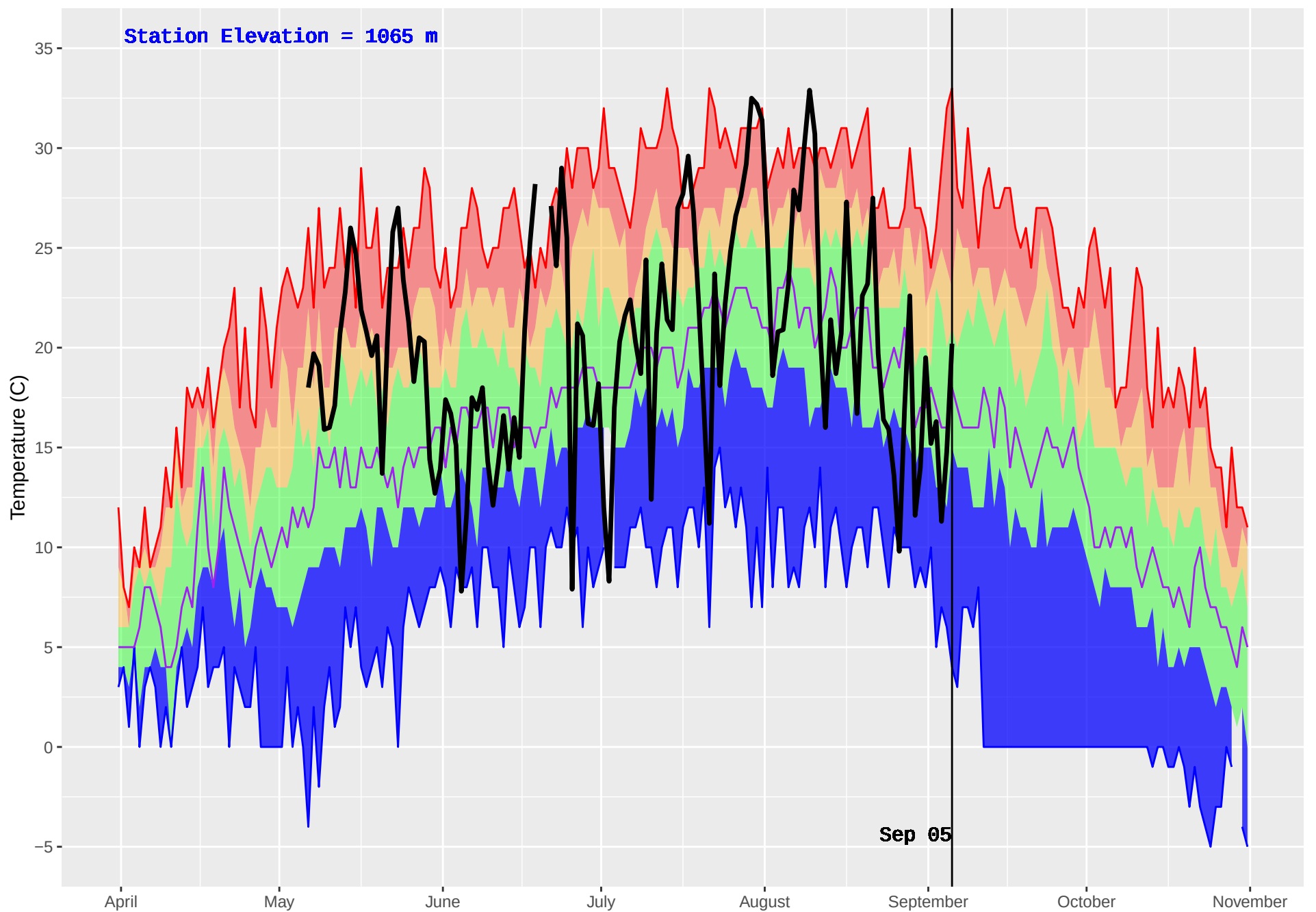
PLACE LAKE (212) : Historical (1981–2016) and Current (2018) Daily Temperature
