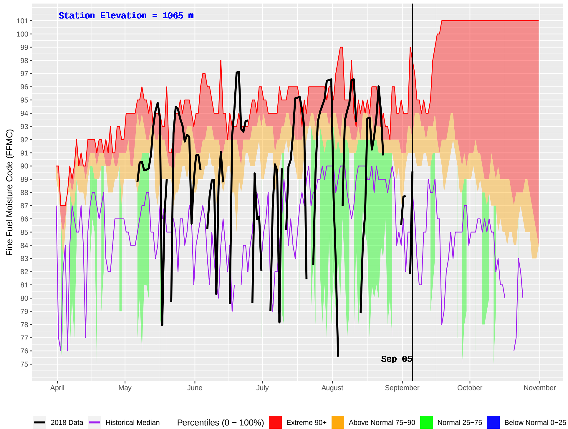
PLACE LAKE (212) : Historical (1981–2016) and Current (2018) Daily Fine Fuel Moisture Code (FFMC)
