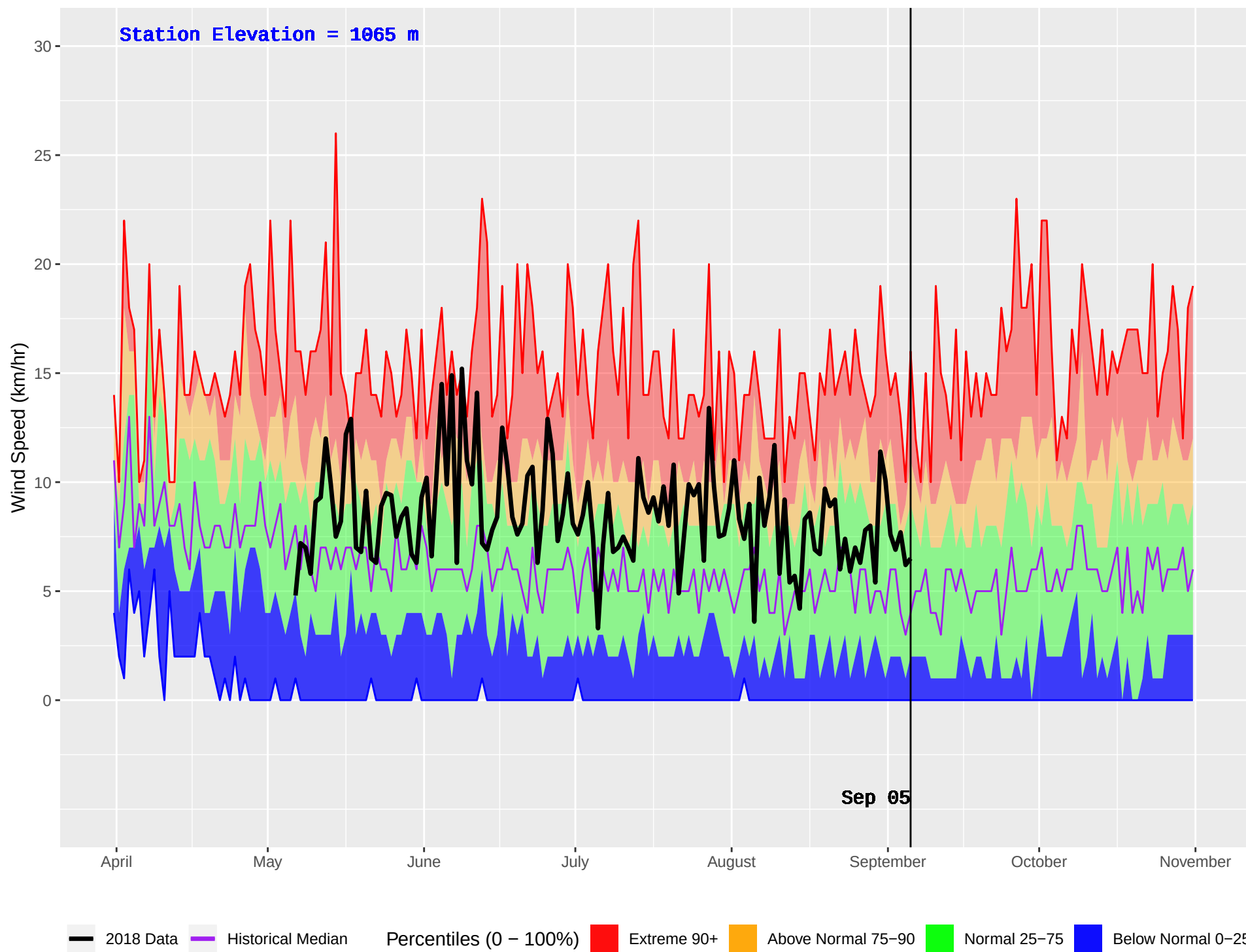
PLACE LAKE (212) : Historical (1981–2016) and Current (2018) Daily Wind Speed
