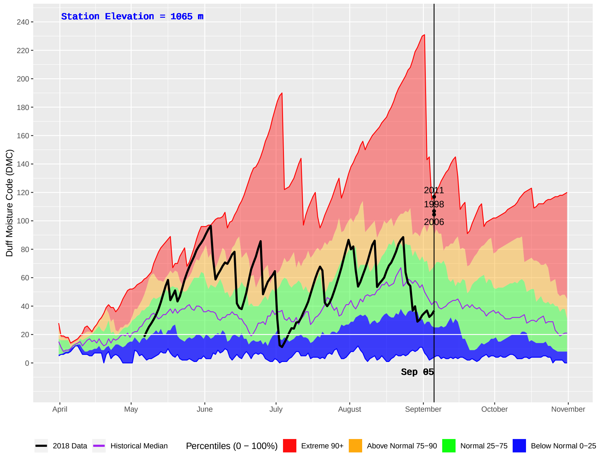
PLACE LAKE (212) : Historical (1981–2016) and Current (2018) Daily Duff Moisture Code (DMC)
